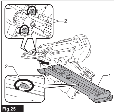
Fig.25 ▶ 1. Magazine 2. Bolts
