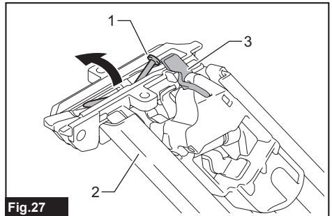
Fig.27 ▶ 1. Jammed fastener 2. Magazine 3. Lock plate
